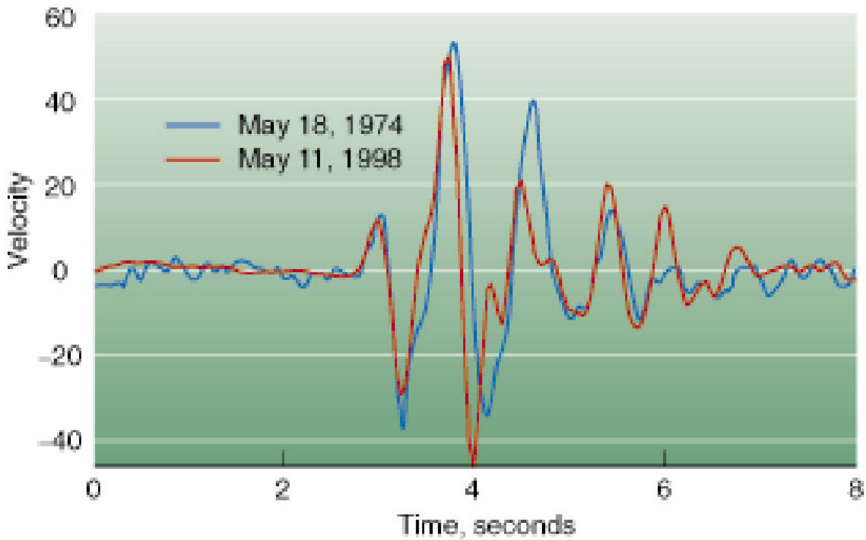
Figure 4. Signals from the 1974 and 1998 Indian underground nuclear tests recorded in northern Canada. (To make the similarities more apparent, the amplitude of the May 18, 1974, data has been doubled.)
