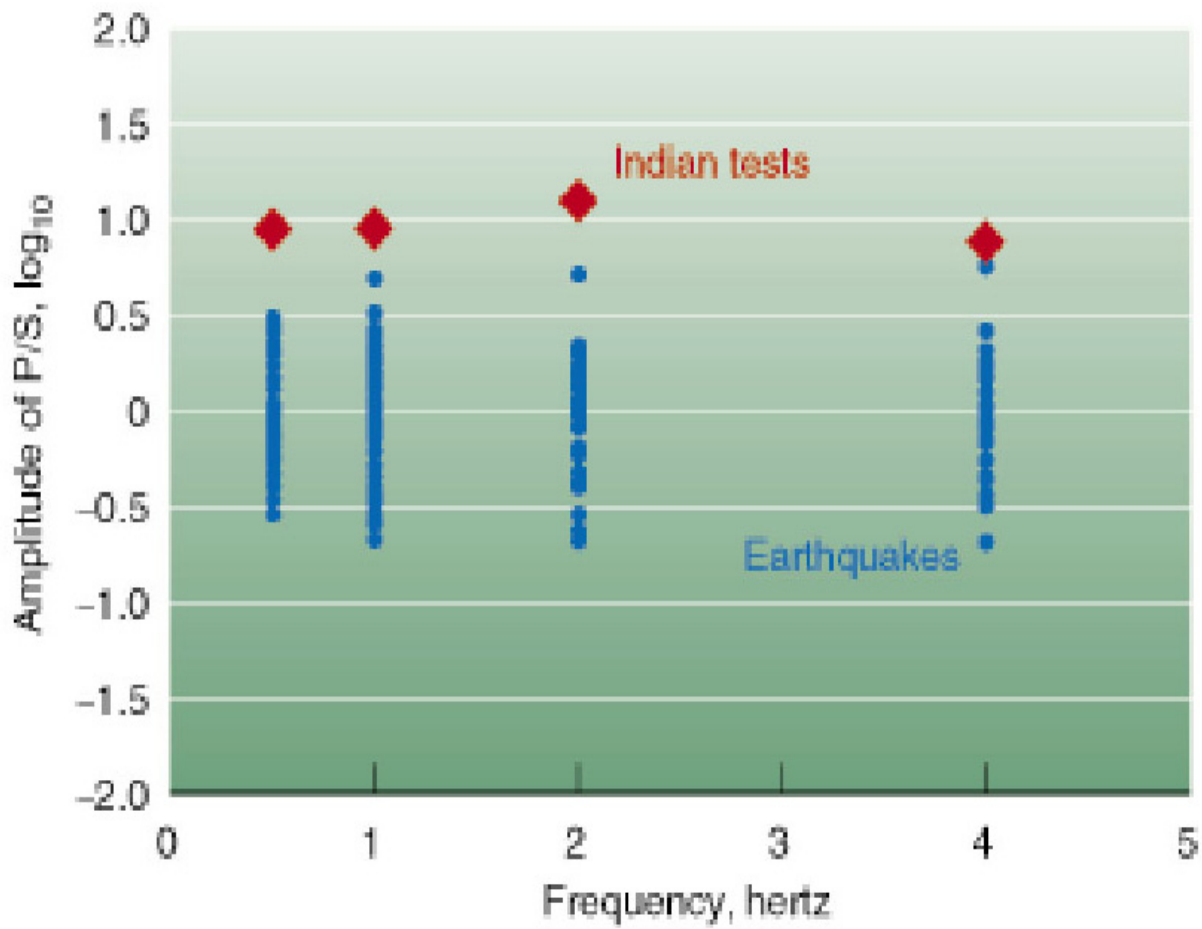
Figure 3. P-to-S amplitude ratios versus frequency for the Indian nuclear test (diamonds) and nearby earthquakes (circles). Note that the P- to S-wave ratios are higher for the Indian test than for the earthquakes.
