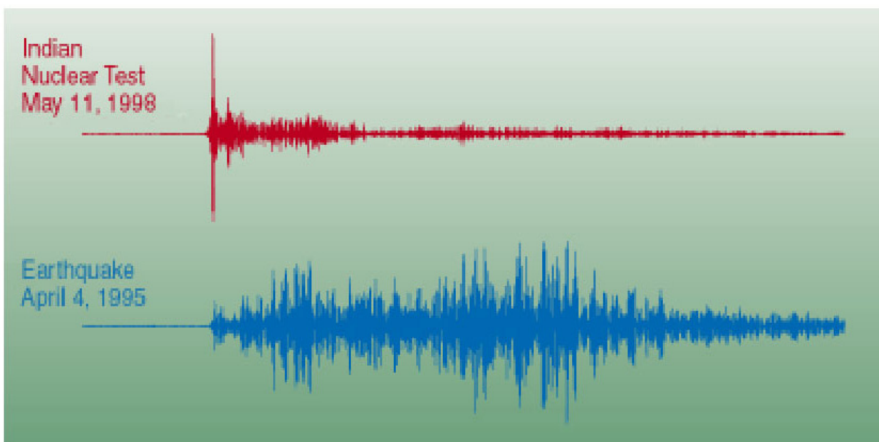
Figure 2. Seismograms of the Indian nuclear test (top) and a representative nearby earthquake (bottom) recorded at the seismic station at Nilore, Pakistan. These seismic signatures for an explosion and earthquake are typical and clearly distinguish one from the other.
