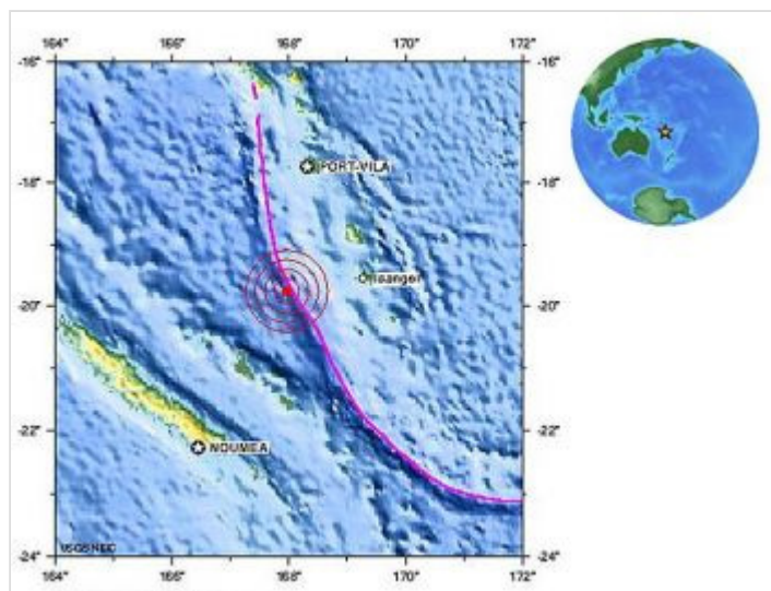
Vanuatu earthquake: The earthquake location map on Dec. 25 at 13:16 UTC time, or 8:15am EST. (USGS.gov)
