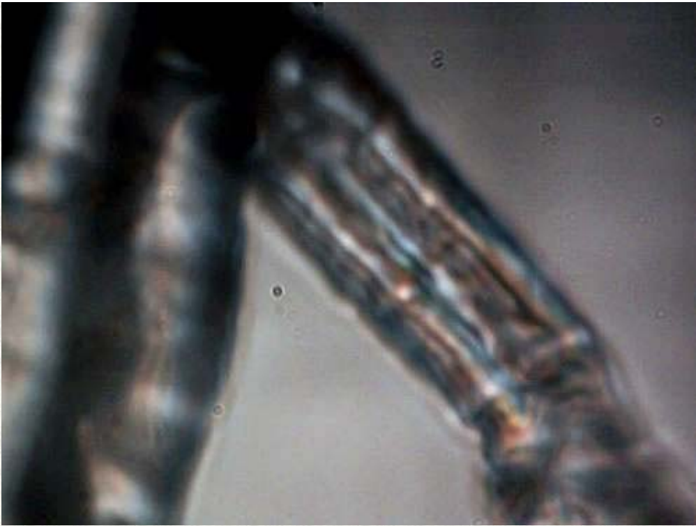
Magnification approximately 5600x. This photograph shows the ability of the fiber to be folded and/or twisted. Internal parallel organization of sub-fibers is visible. Non-uniformity of the fibers dimensions is also evident. Transverse separation or structure also visible in lower right of image.
